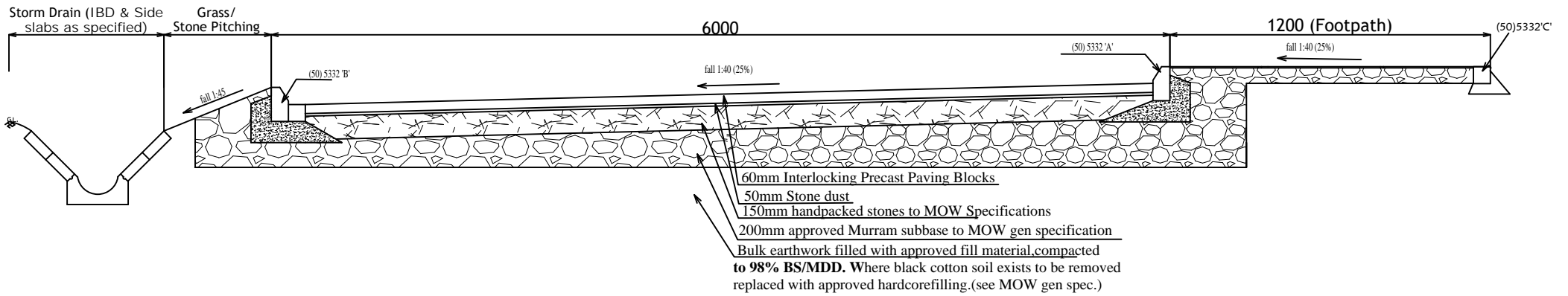
TYPICAL ROAD CROSS SECTION - (ONE WAY FALL)
